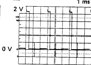
Slight positive step at -0.6 V only present in MIX. Positive spike at -0.6 V is higher in A INTEN and B DLY'D modes.
